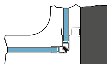
Detail A - pohled shora
